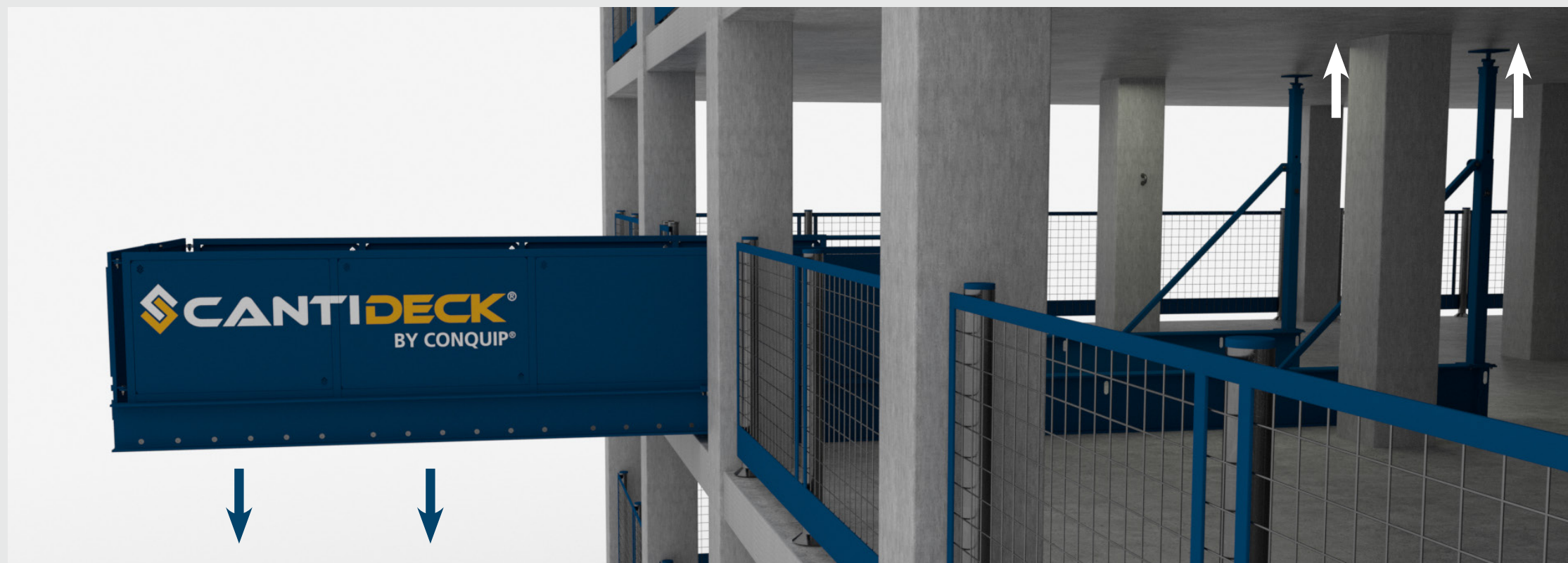
03 / A simple propping mechanism secures the deck into the structure.
