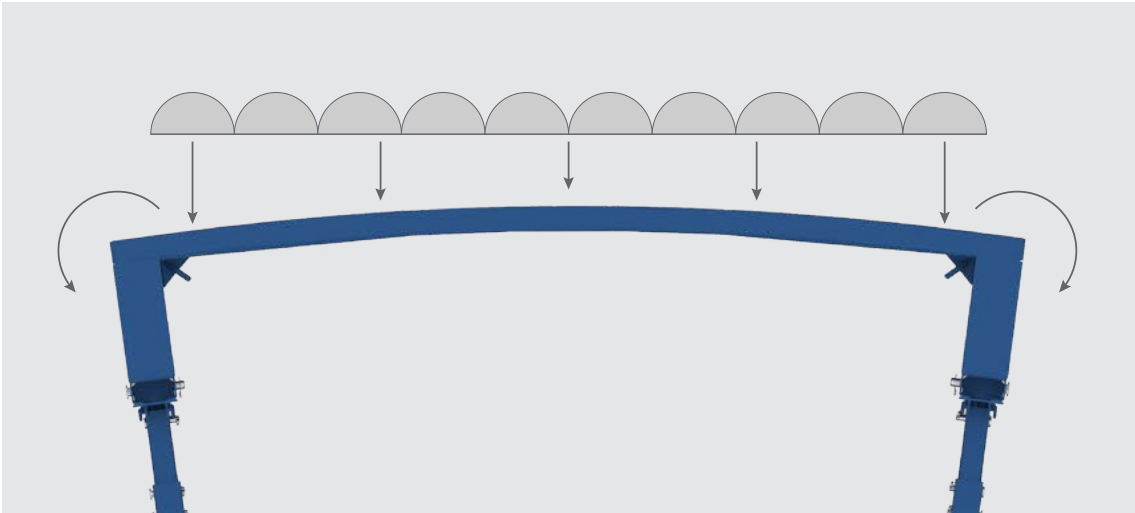
CORNER MOMENT
